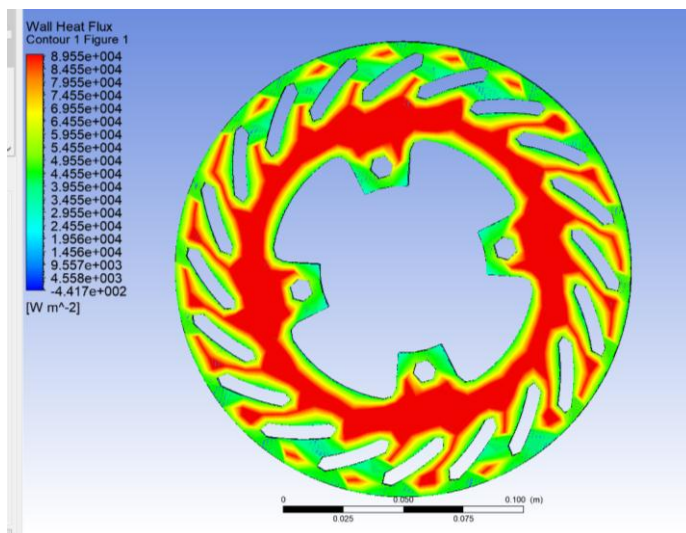
Fig -8: Wall Heat Flux distribution around the disc
