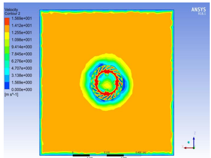
Fig -9: Velocity of air around the disc
