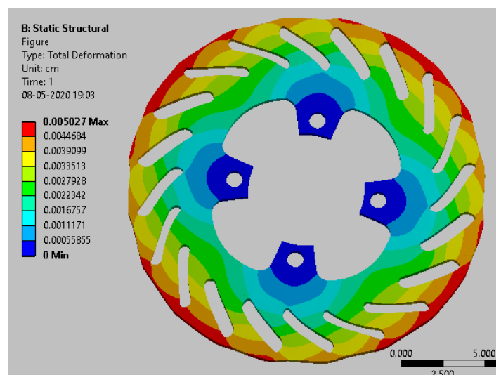
Fig -11: Total Deformation
