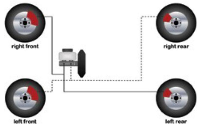
Fig -1: X -Split braking Circuit
